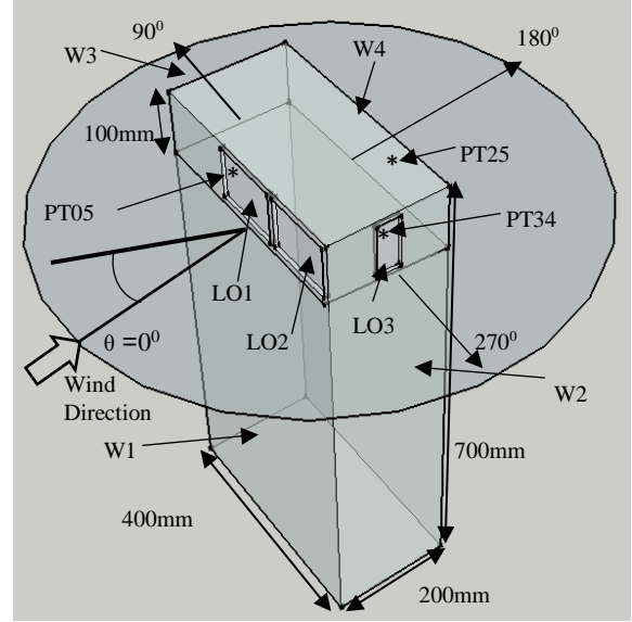
Figure 1. 1:200 Scale wind tunnel model.
