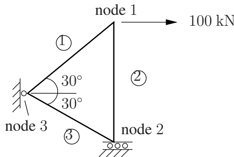
FIGURE 5.2: A system of three trusses.
