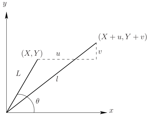
FIGURE 5.1: A truss of initial length L is stretched to a new length l . Displacements of the right hand end relative to the left hand end are u and v in the x - and y - directions, respectively.
