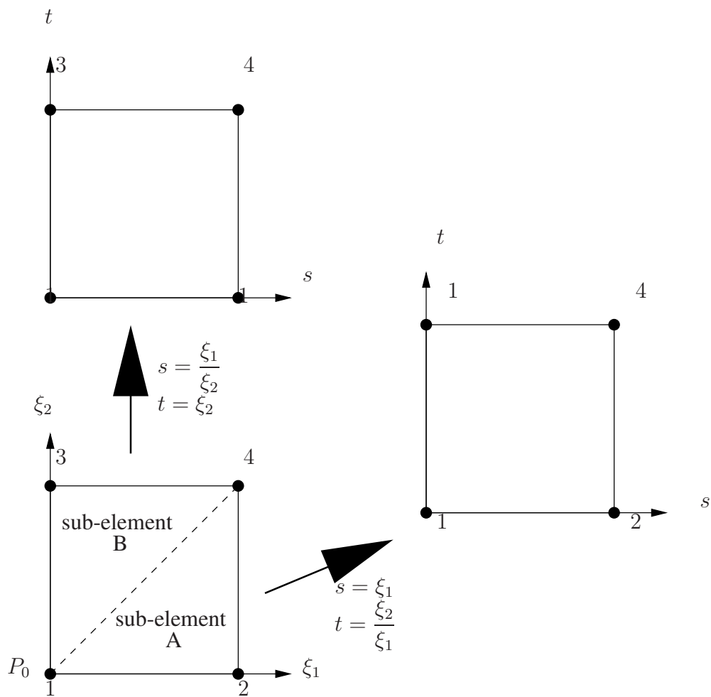
FIGURE 7.1: The element splitting used when P_0 is at local node 1. The individual transformations yield Jacobians that reduce the order of the singularity in the otherwise singular boundary element integrals.
