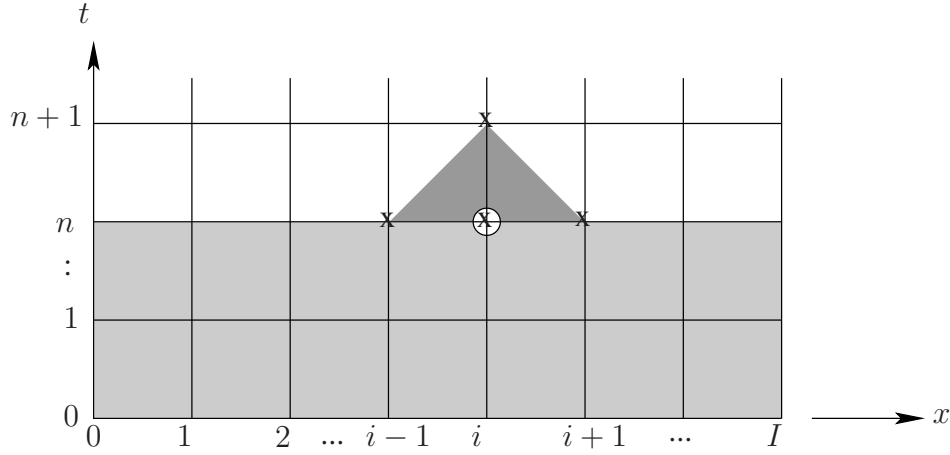
FIGURE 4.1: A finite difference grid for the solution of the transient 1D heat equation. The equation is centred at grid point (i, n) shown by the \bigcirc . The lightly shaded region shows where the solution is known at time step n . With central differences in x and a forward difference in t an explicit finite difference formula gives the solution at time step n + 1 explicitly in terms of the solution at the three points below it at step n , as indicated by the dark shading.
