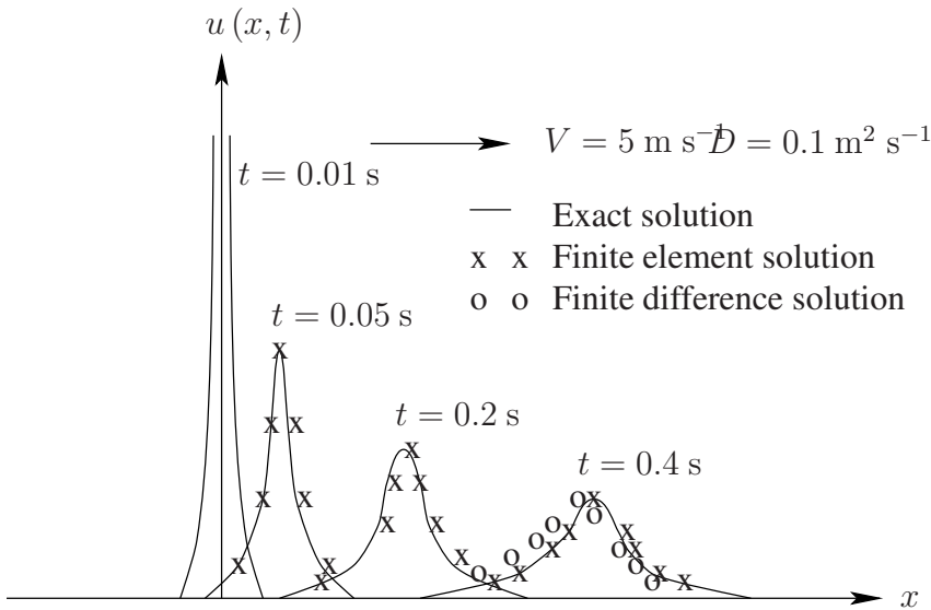
FIGURE 4.4: Advection-diffusion of a unit mass pulse. The finite element solutions (at t=0.01 s, 0.05 s, 0.2 s and 0.4 s) and finite difference solutions (at t=0.4 s only) are compared with the exact solution. \Delta x=0.1 , \Delta t=0.001 s for 0 < t < 0.01 s and \Delta t=0.01 for t \geq 0.01 s.
