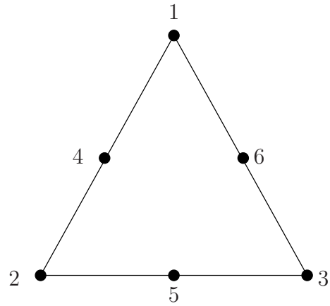
FIGURE 1.16: Basis functions for a six node quadratic triangular element.
