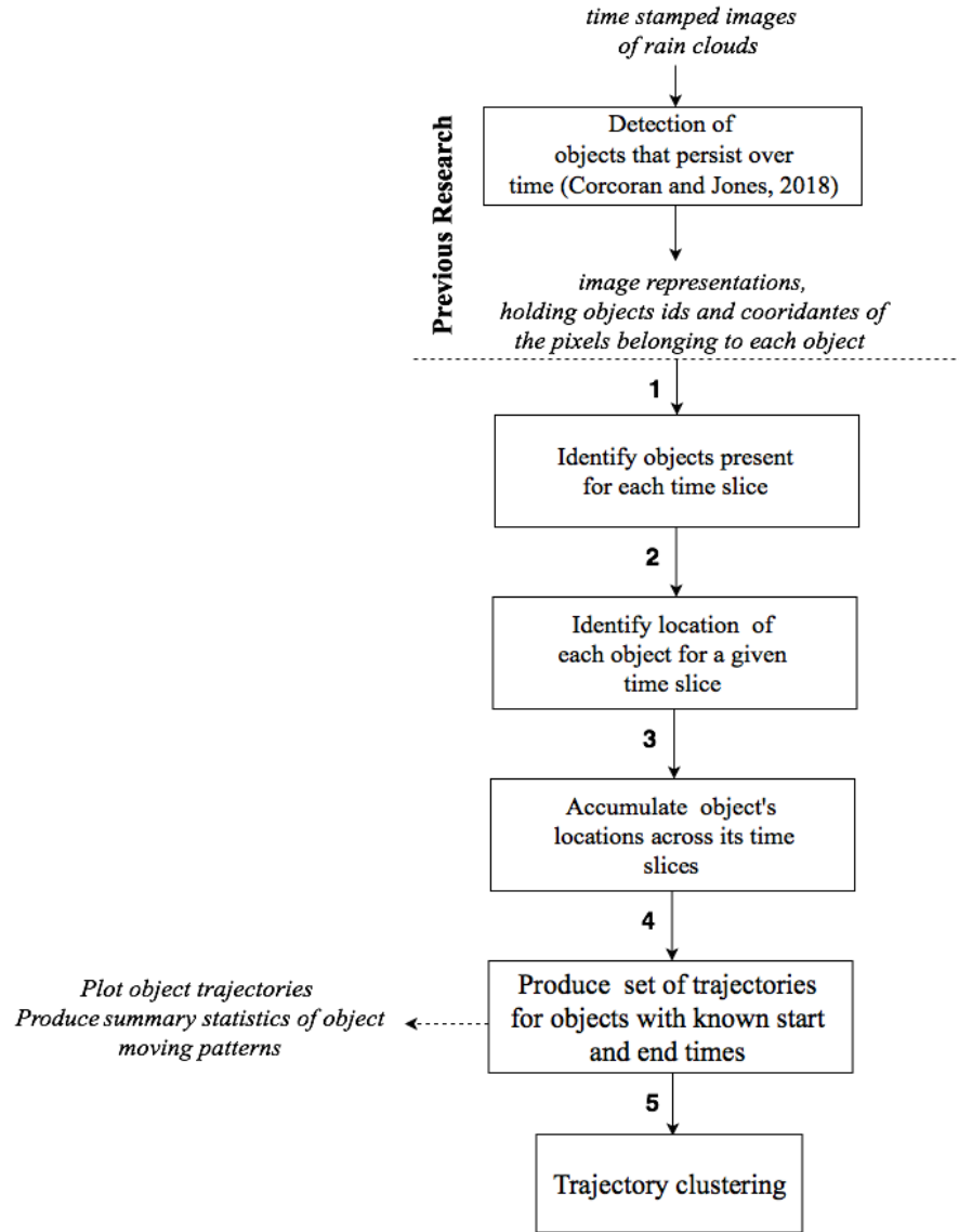
Figure 1: Methodology overview
