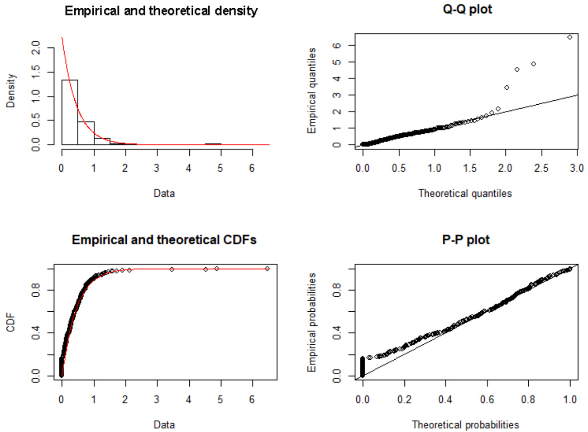
Figure 5: Empirical and theoretical densities (top-left), Q-Q plot (top-right), Cumulative Distribution Function (CDF) (bottom-left) and the P-P plot (bottom-right) of exponential distribution of negative class of sentiment scores.
