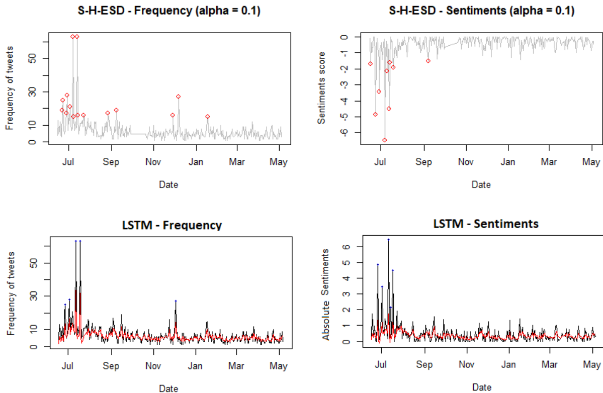
Figure 6: S-H-ESD anomaly detection for the frequency of tweets (top-left) and sentiments scores (top-right), LSTM anomaly detection for the frequency of tweets (bottom-left) and sentiments scores (bottom-right). The value of \alpha is set based on experiments and better recall and precision values.
