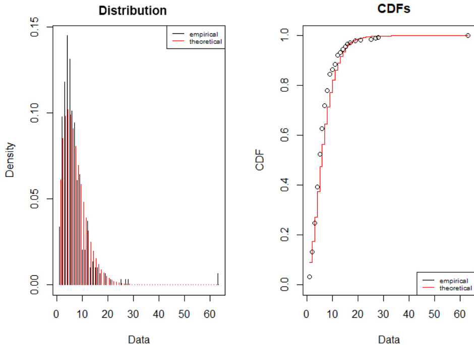
Figure 4: Empirical and theoretical distribution (left) and Cumulative Distribution Function (CDF) (right) of frequency data using negative binomial distribution.
